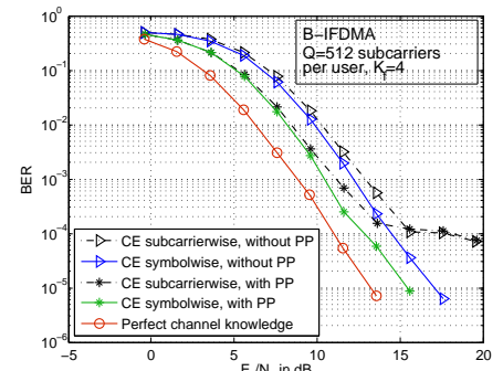
Figure 5: B-IFDMA with realistic CE
