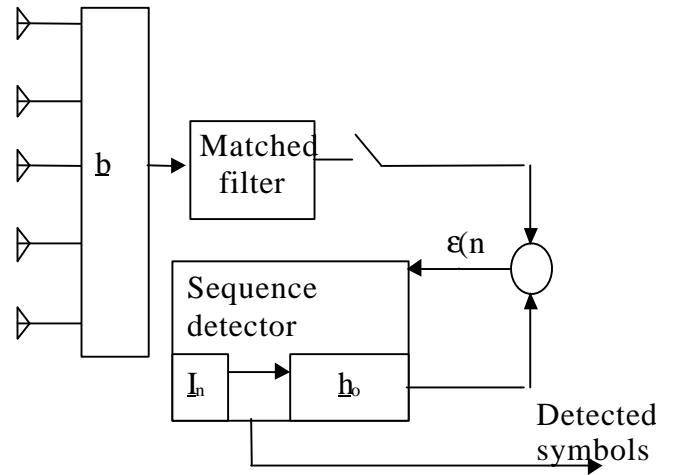
Figure 1. Spatial diversity processing with sequence detector.
