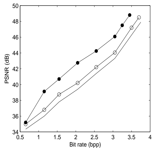
Figure 3: PSNR (in dB) versus the bit rate (bpp) after EZBC encoding for the SI pair "spot5-2": 5/3 for (I^{(l)}, I^{(e)}) in solid line, 5/3 for (\tilde{I}, I^{(e)}) in line with circle, VLS-II in dots.
